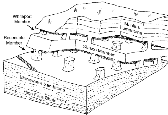
FIG. 8—A three-dimensional sketch of the inner workings of a typical room-and-pillar mine in the Rosendale natural cement region. Cement rocks were extracted from the Rosendale and Whiteport members of the Rondout Formation (see also Fig. 7). Rocks in the Glasco Member of the Rondout Formation were unsuitable for cement production and were commonly not removed, resulting in a ledge that separated the two mined horizons. Mining of cement rocks began with the excavation of a series of rooms in the Rosendale or Whiteport members, or both along a surface exposure. Subsequent mining interconnected these rooms at depth, leaving pillars of cement rock to support the weight of overlying strata. The initial rooms were then extended with new shafts, which were later interconnected to form a new row of rooms and pillars.
